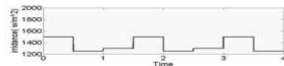
Figure 5. Solar irradiation.
