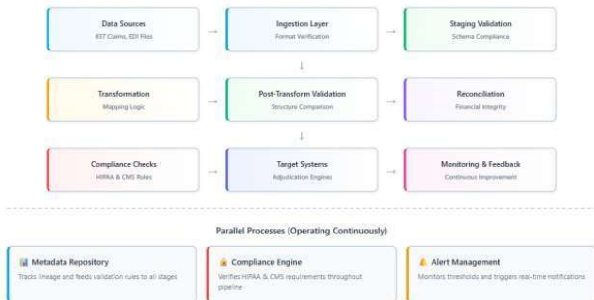
Figure 1: Intelligent ETL Validation Pipeline Architecture
